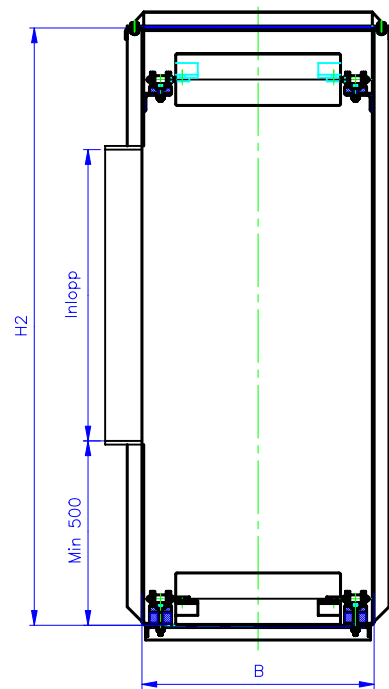
Snitt B-B Typ: TKF...HBL
